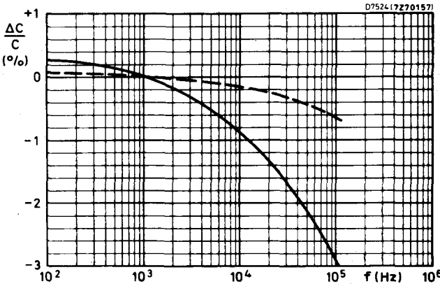
Typical capacitance change as a function of frequency
