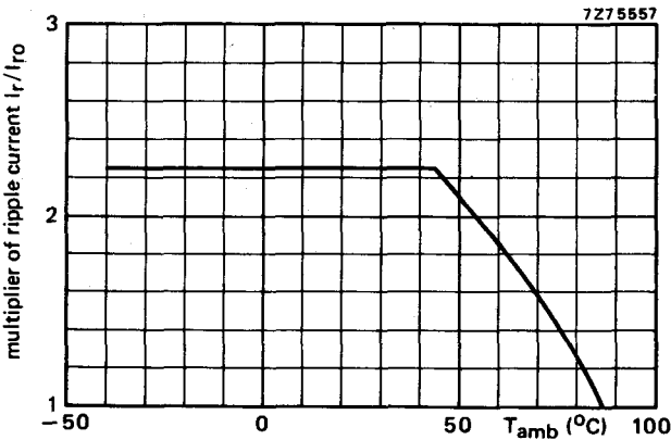
Fig. 2 Typical ripple current as a function of ambient temperature; I_{r0} = ripple current at 85 °C; 100 Hz.
