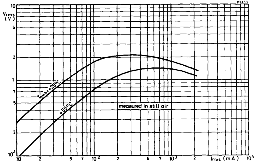
VOLTAGE/CURRENT CHARACTERISTICS
