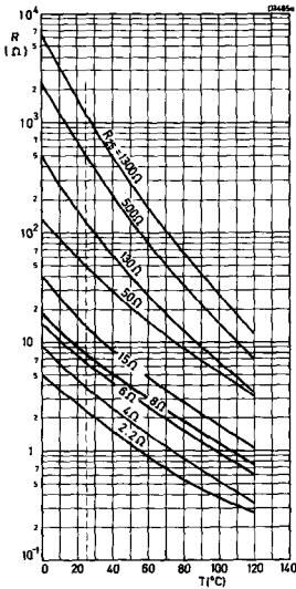
Resistance/temperature characteristics
