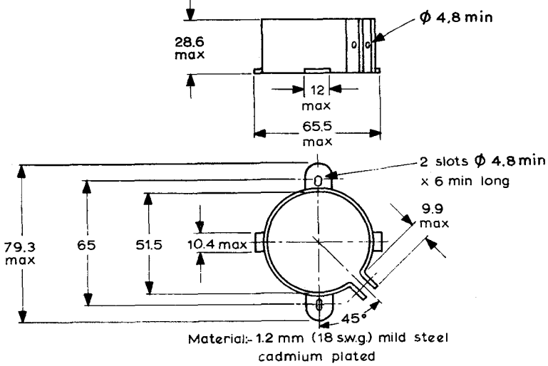
Fig.3 Clamp for case diameter of 50 mm Type No. DT2254
