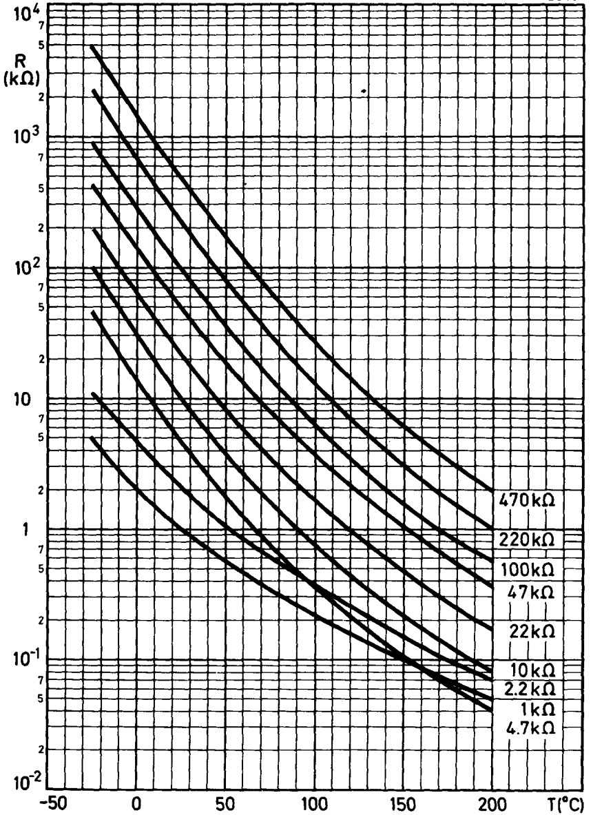
RESISTANCE/TEMPERATURE CHARACTERISTICS FOR VA 3100, VA 3200, VA 3400, VA 3700 SERIES
