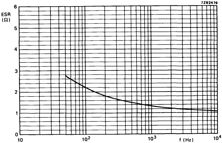
Fig. 16 Typical ESR as a function of frequency at 20 °C. Case size 04: 47 μF, 350 V.
