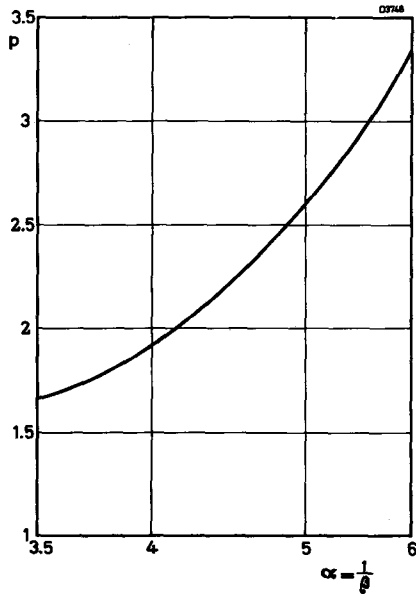
Fig. 9 Relation between the power dissipation caused by a d. c. voltage V and an a. c. voltage V_{r.m.s.} = V
