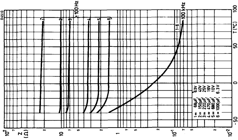
Impedance plotted against temperature with frequency as a parameter. Can size 01
