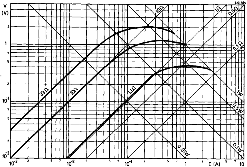
Voltage/current characteristics
