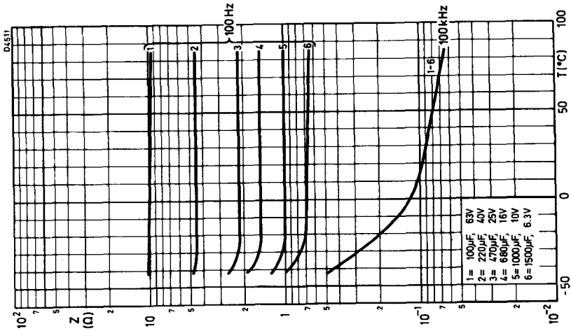
Impedance plotted against temperature with frequency as a parameter. Can size 02
