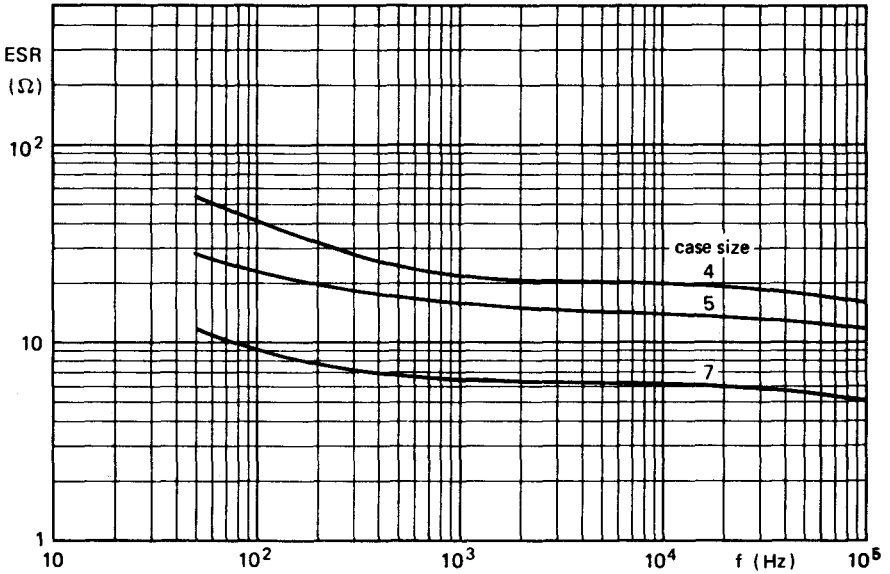
Fig. 8 Typical ESR as a function of frequency at 20 °C; U_R = 250 V.
