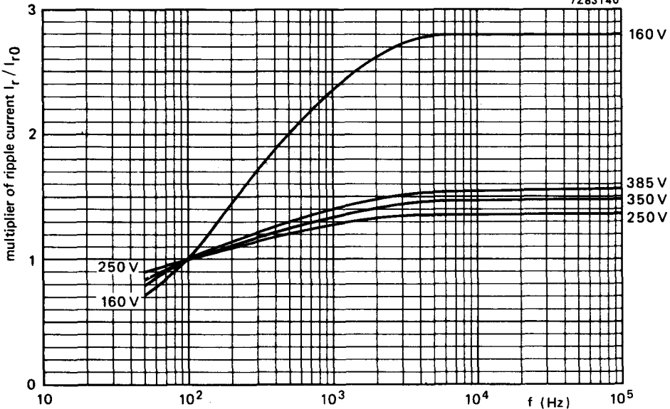
Fig. 6 Typical ripple current as a function of frequency; I_{r0} = ripple current at 85 °C, 100 Hz.
