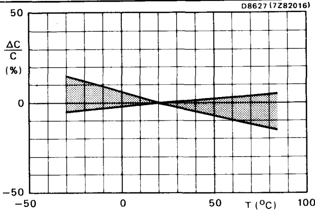
Fig.7 Characteristic X (2C2, Y5R)
