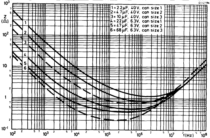
IMPEDANCE PLOTTED AGAINST FREQUENCY AT T_{amb} = 20^{\circ}C (CAN SIZES 1, 2 AND 3)
