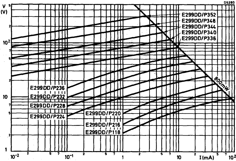
VOLTAGE/CURRENT CHARACTERISTICS
