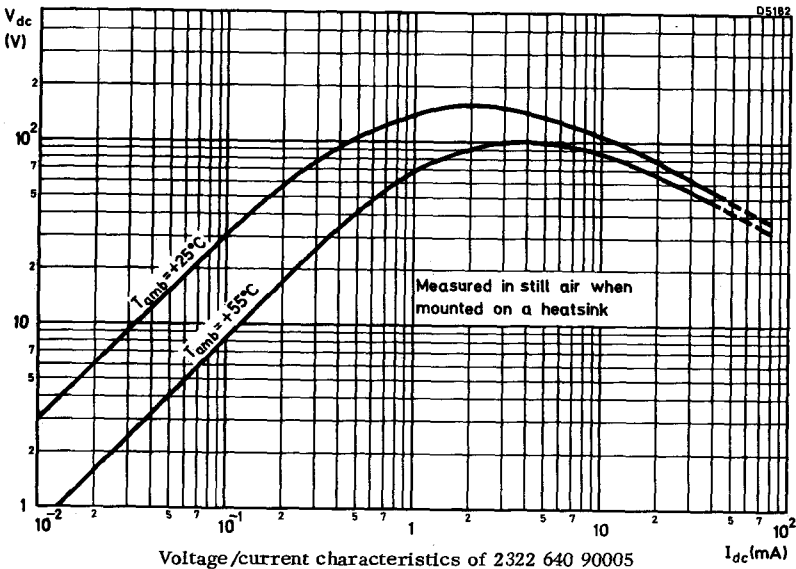
Voltage/current characteristics of 2322 640 90005
