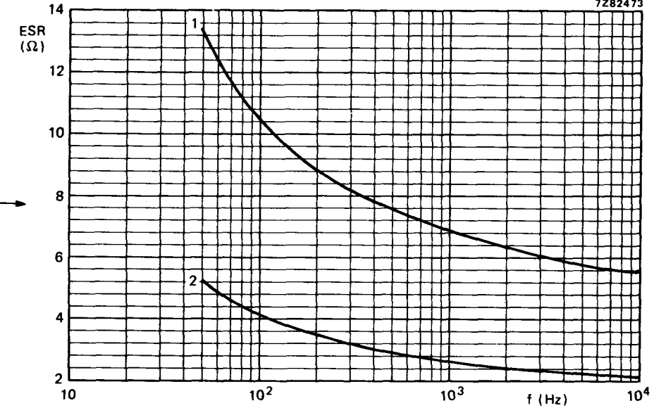
Fig. 13 Typical ESR as a function of frequency at 20 °C. Case size 01: curve 1 = 10 μF, 350 V/385 V; curve 2 = 22 μF, 250 V.
