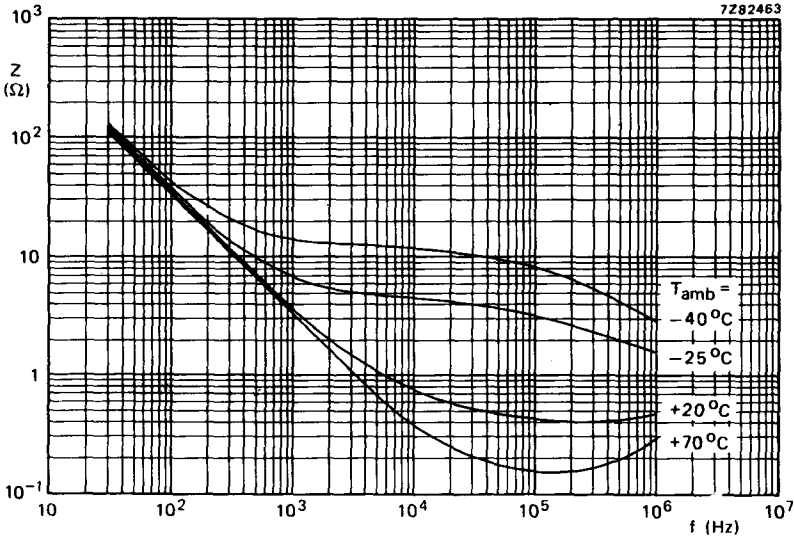
Fig. 19 Typical impedance as a function of frequency at different temperatures. Case size 02: 47 \mu F, 160 V.
