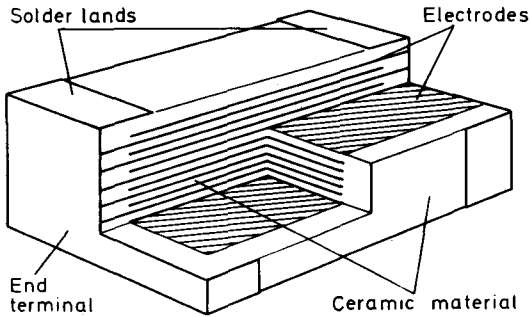
Fig. 1 Cross-section of a multilayer chip capacitor
