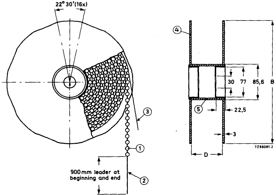
Fig.3 Reel dimensions (mm) B = 305; D = 75
