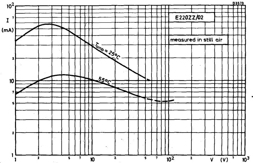
VOLTAGE/CURRENT CHARACTERISTICS
