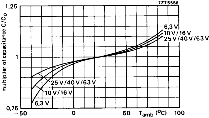
Fig. 3 Typical capacitance as a function of ambient temperature; C_0 = capacitance at 25 ^{\circ}\text{C} , 100 Hz.
