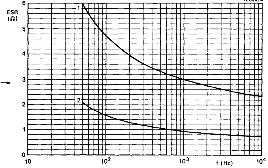
Fig. 14 Typical ESR as a function of frequency at 20 °C. Case size 02: curve 1 = 22 μF, 350 V; curve 2 = 47 μF, 160 V.
