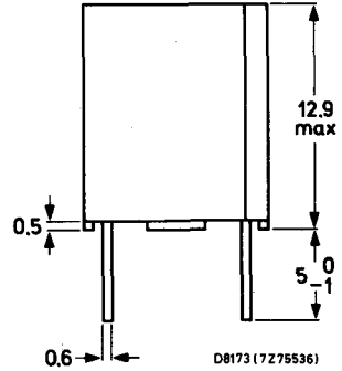
Fig.2 Capacitors of rated capacitance range 15 400 to 34 000 pF.
