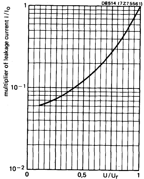
Fig.10 Typical leakage current as a function of U/U_R ; I_0 = leakage current during continuous operation at 25 ^{\circ}\text{C} and U_R .
