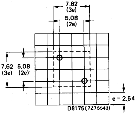
Fig.3 Required space for capacitors according to Fig.1
