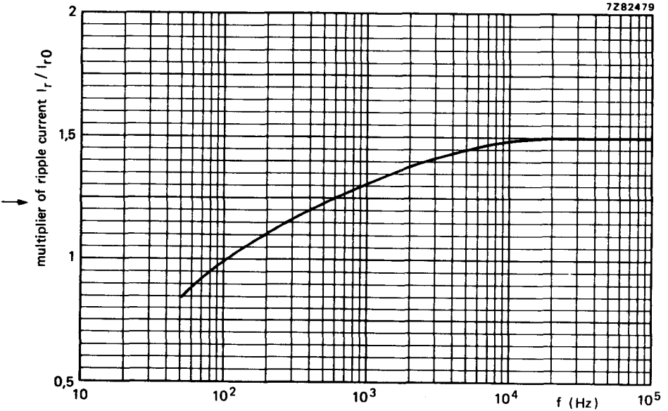
Fig. 6 Typical ripple current as a function of frequency; I_{r0} = ripple current at 70\text{ }^{\circ}\text{C} , 100 Hz.
