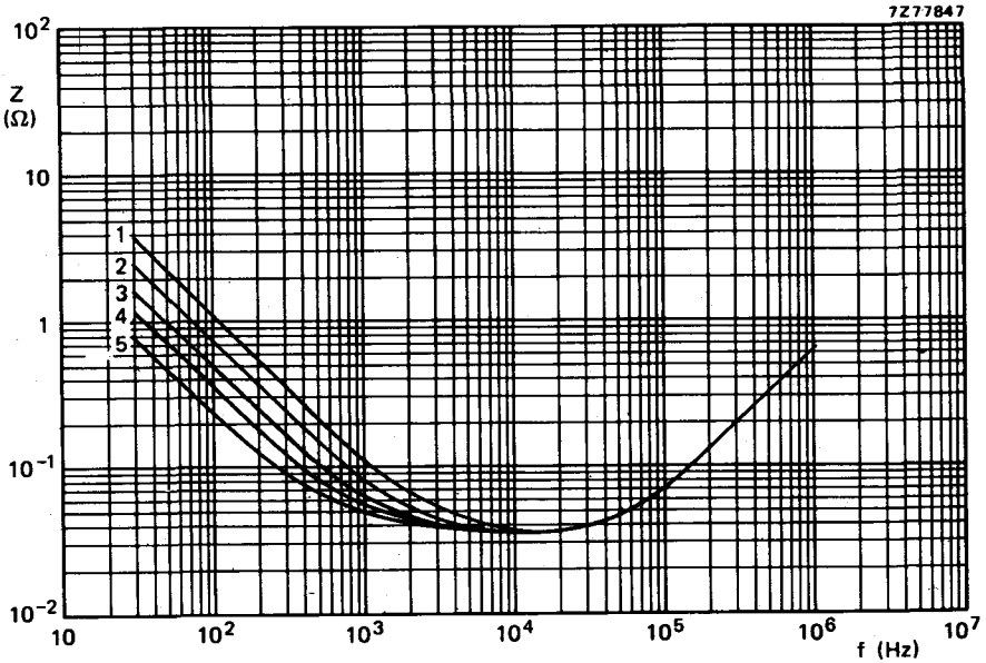
Fig. 13 Typical impedance as a function of frequency at 25 °C. Case size 04: curve 1 = 1500 \mu\text{F} , 40 V; curve 3 = 3300 \mu\text{F} , 16 V; curve 5 = 6800 \mu\text{F} , 6,3 V. curve 2 = 2200 \mu\text{F} , 25 V; curve 4 = 4700 \mu\text{F} , 10 V;
