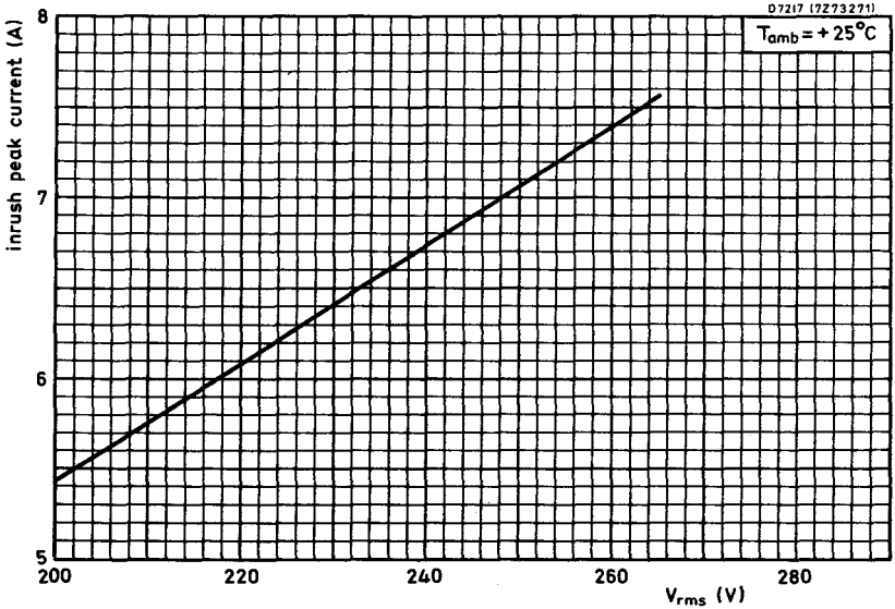
Fig. 5. Typical inrush peak current versus voltage characteristic
