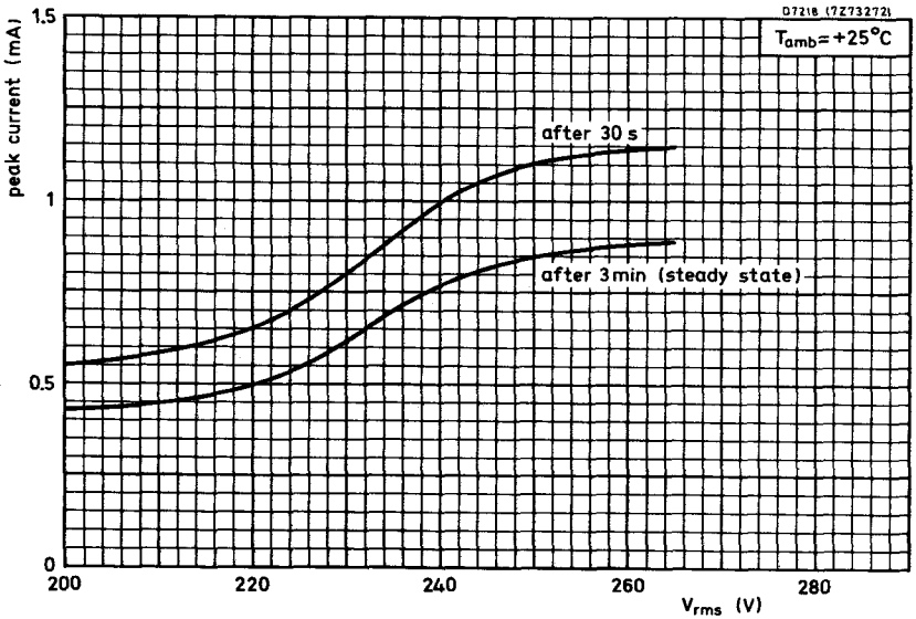
Fig. 6. Typical peak current versus voltage characteristics.
