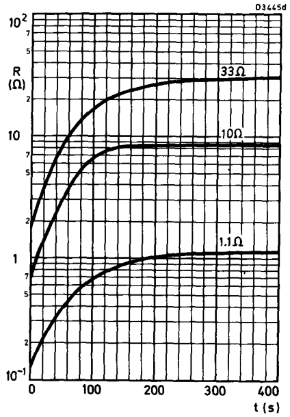
Cooling characteristics
