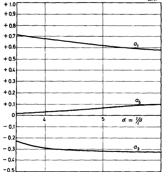
Fig. 12 Relative strengths of the harmonics
