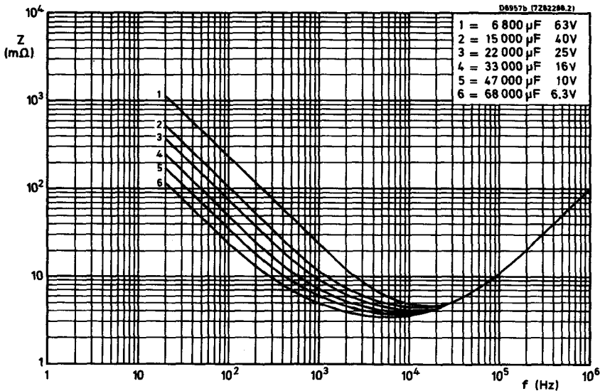
Typical impedance plotted against frequency at T_{\text{amb}} = 20^\circ\text{C} , can size 15
