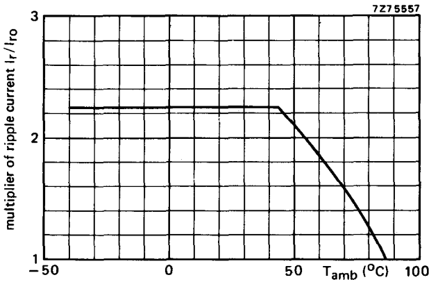
Fig. 5 Typical ripple current as a function of ambient temperature; I_{r0} = ripple current at 85 °C, 100 Hz.
