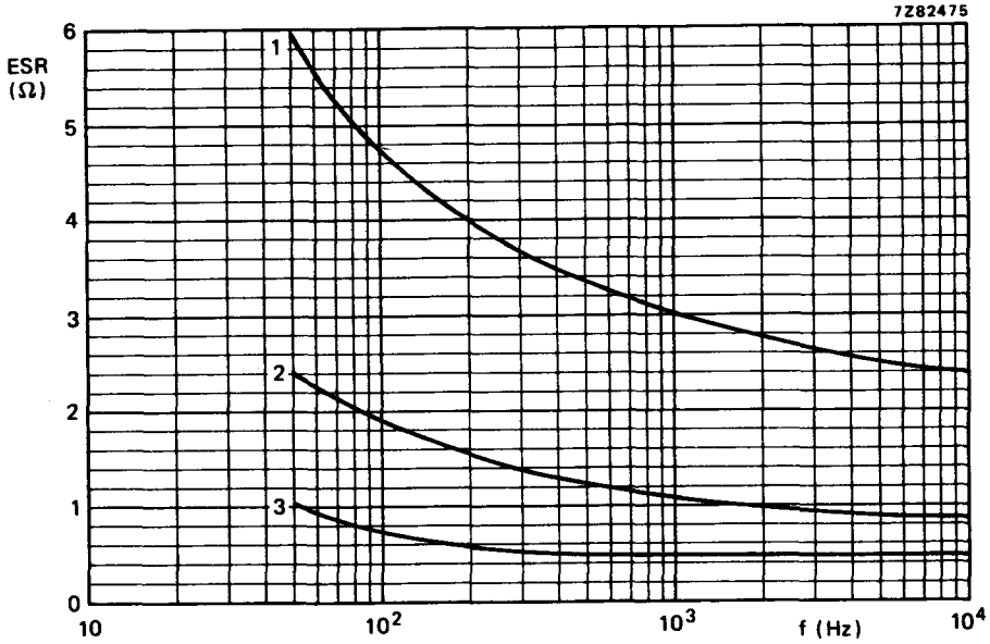
Fig. 15 Typical ESR as a function of frequency at 20 °C. Case size 03: curve 1 = 22 μF, 385 V; curve 2 = 47 μF, 250 V; curve 3 = 100 μF, 160 V.
