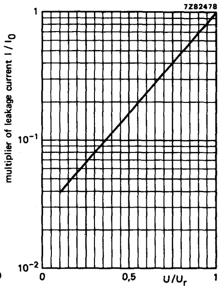
Fig. 8 Typical leakage current as a function of U/U_R ; I_0 = leakage current during continuous operation at 25 °C and U_R .
