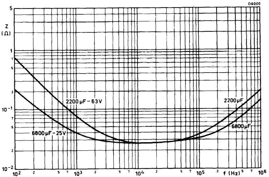
Typical impedance plotted against frequency. T_{amb} = 20\text{ }^{\circ}\text{C}
