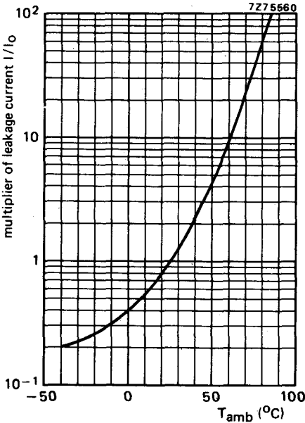
Fig. 7 Typical leakage current as a function of ambient temperature; I_0 = leakage current during continuous operation at 25\text{ }^{\circ}\text{C} and U_R .
