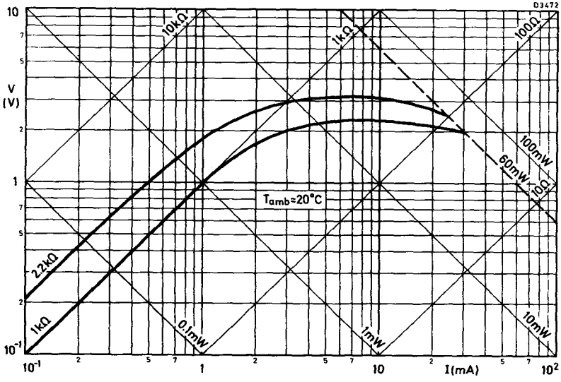
VOLTAGE/CURRENT CHARACTERISTICS FOR VA3200 SERIES ONLY
