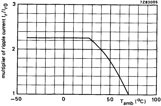
Fig. 5 Typical ripple current as a function of ambient temperature; I_{r0} = ripple current at 70\text{ }^{\circ}\text{C} , 100 Hz.
