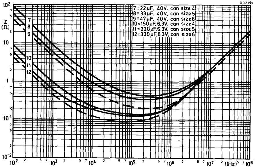
IMPEDANCE PLOTTED AGAINST FREQUENCY AT T_{amb} = 20^{\circ}C (CAN SIZES 4, 5 AND 6)
