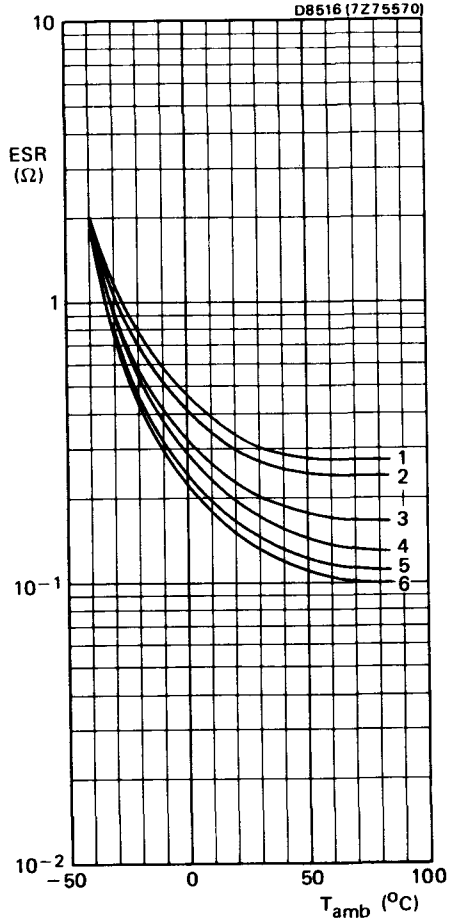
Fig.12 Typical ESR as a function of ambient temperature at 100 Hz
