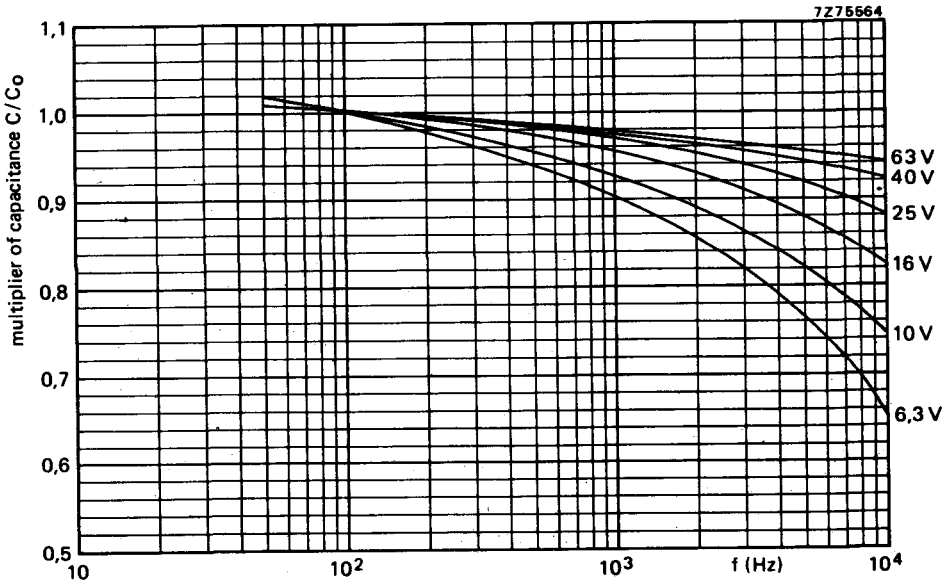
Fig. 4 Typical capacitance as a function of frequency; C_0 = capacitance at 25 ^{\circ}\text{C} , 100 Hz.
