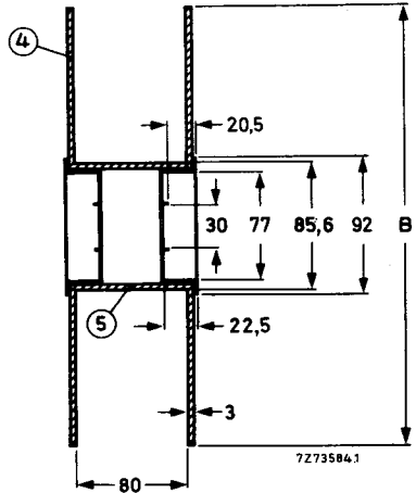
Fig.3 1: capacitor 2: bandolier 3: paper 4: flange 5: cylinder
