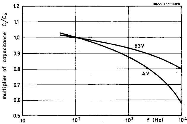
Fig.9 Typical capacitance as a function of frequency
