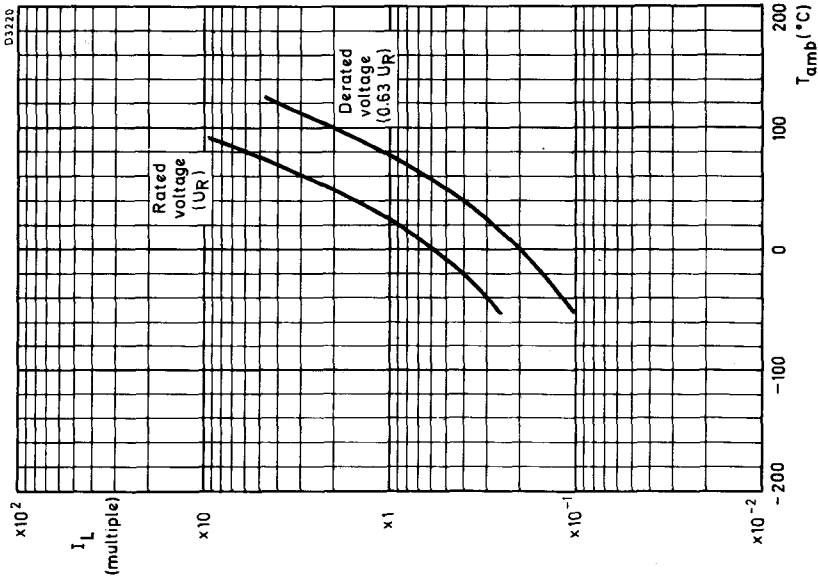
MULTIPLE OF LEAKAGE CURRENT ( I_L for T_{amb} = 20^\circ C ) PLOTTED AGAINST AMBIENT TEMPERATURE
