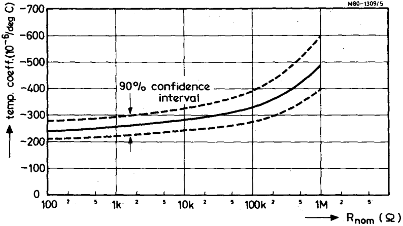
Fig.5 Temperature coefficient as a function of the resistance value
