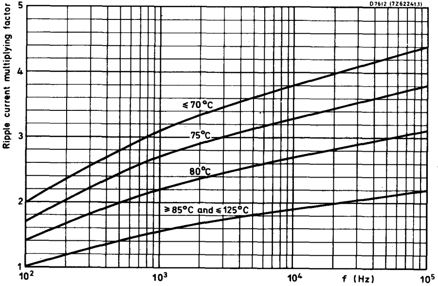
TYPICAL RIPPLE CURRENT MULTIPLYING FACTOR PLOTTED AGAINST FREQUENCY
