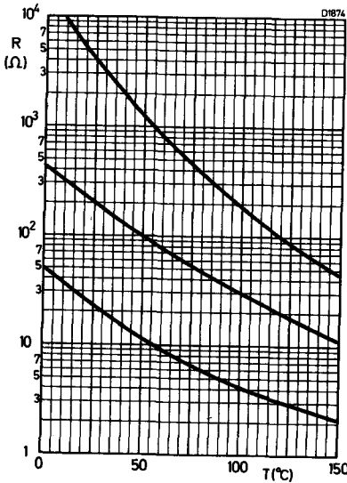
Fig. 1 Resistance as a function of temperature for three different values of A and B
