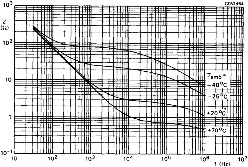
Fig. 20 Typical impedance as a function of frequency at different temperatures. Case size 02: 22 \mu F, 350 V.
