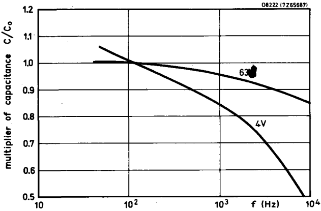
Fig.8 Typical capacitance as a function of frequency
