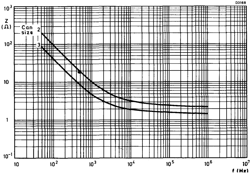
Fig.6 Typical impedance plotted against frequency, T_{amb} = 20^{\circ}C
