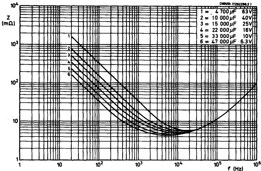
Typical impedance plotted against frequency at T_{\text{amb}} = 20^\circ\text{C} , can size 14
