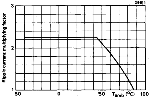
Fig. 7 Typical ripple current as a function of ambient temperature at 100 Hz
