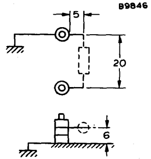
Fig.7 Measuring arrangements
