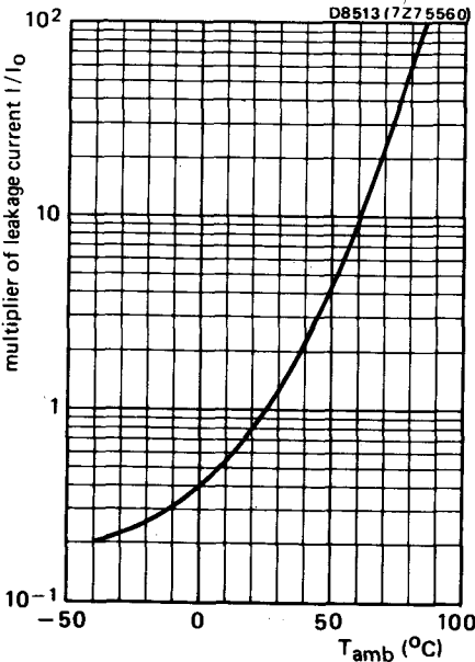
Fig.9 Typical leakage current as a function of ambient temperature; I_0 = leakage current during continuous operation at 25 ^{\circ}\text{C} and U_R .
