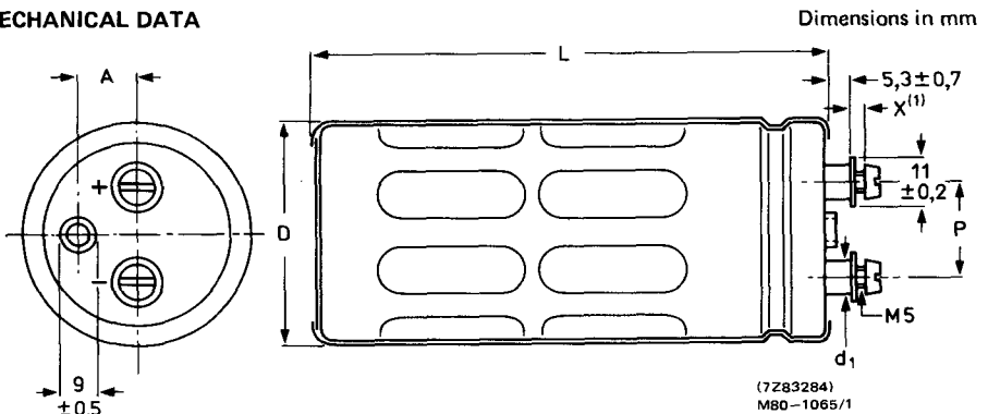
Fig.1 See Table 1 for dimensions D, L, P, A, d 1 , d 2 , and l.
