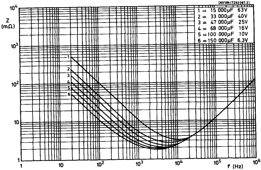
Typical impedance plotted against frequency at T_{amb} = 20\text{ }^{\circ}\text{C} , can size 16
