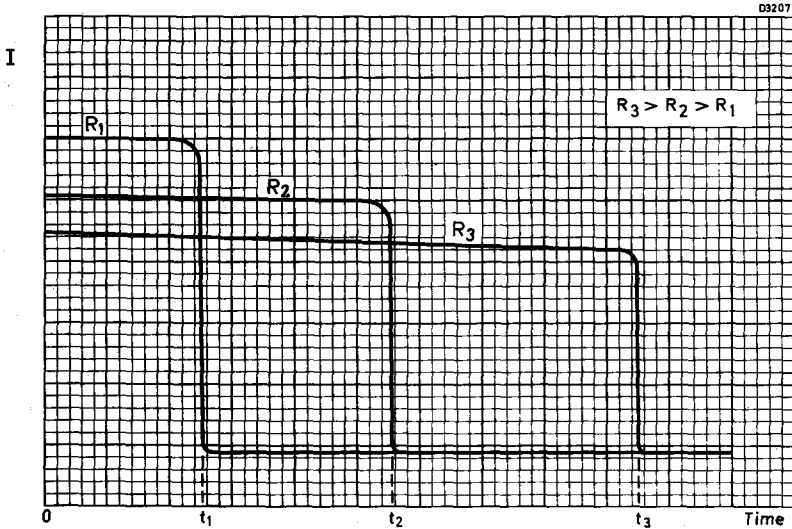
Fig. 9 The influence of resistance value on the current/time characteristic of a p.t.c. thermistor/resistor combination
