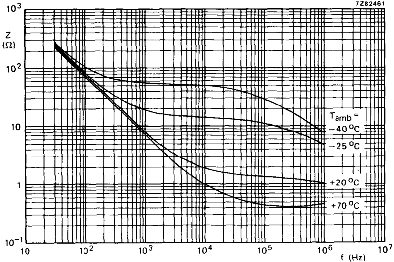
Fig. 17 Typical impedance as a function of frequency at different temperatures. Case size 01: 22 \mu F, 250 V.
