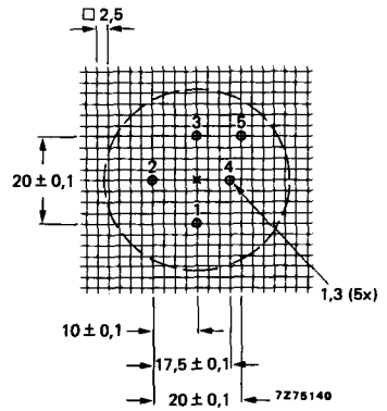
Piercing diagram viewed from component side
