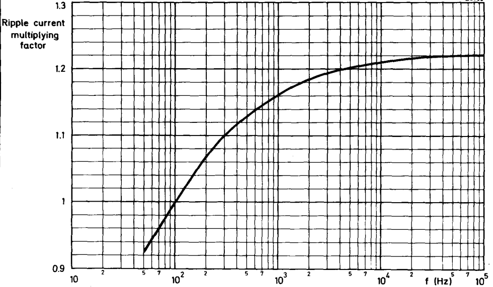
Typical ripple current multiplying factor plotted against frequency
