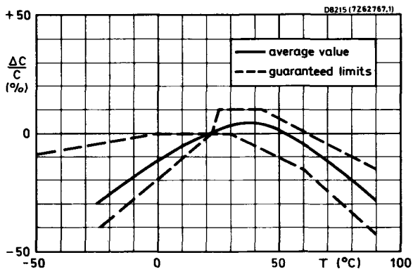
Capacitance change as a function of temperature.
