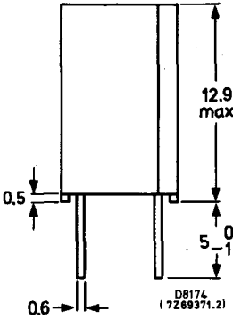
Fig.1 Capacitors of rated capacitance range 100 to 15 000 pF.
