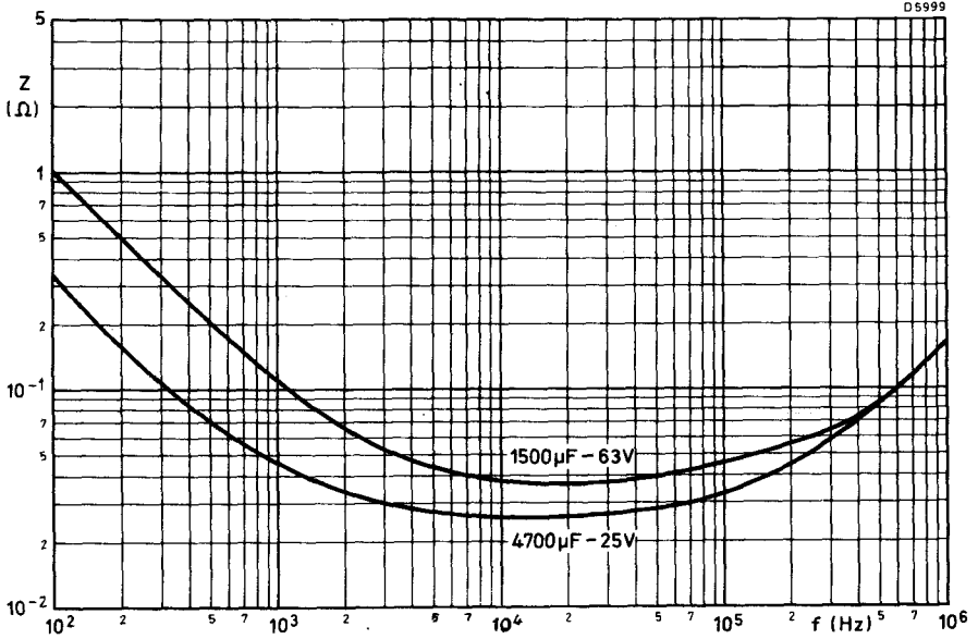
Typical impedance plotted against frequency. T_{amb} = 20\text{ }^{\circ}\text{C}
