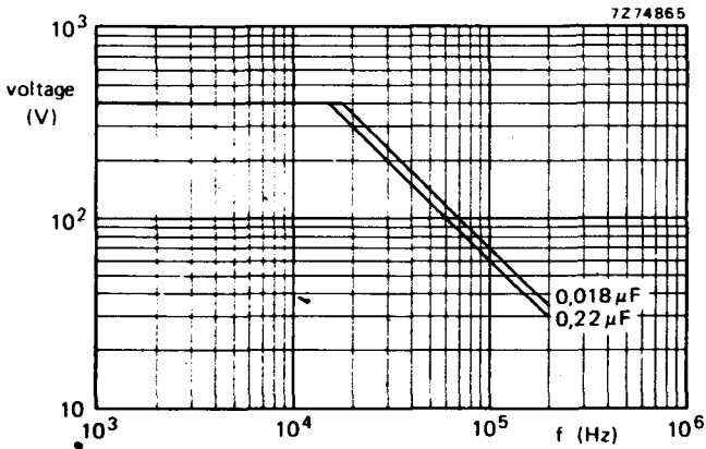
Fig. 4 Maximum permissible r.m.s. value of sinusoidal voltages as a function of frequency at T_{amb} \leq 70^\circ C , for 1000 V version.
