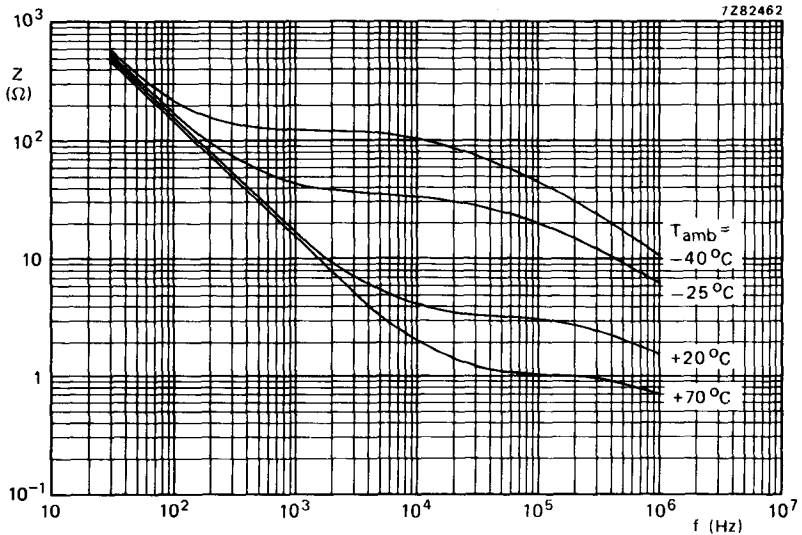
Fig. 18 Typical impedance as a function of frequency at different temperatures. Case size 01: 10 \mu F, 350 V/385 V.
