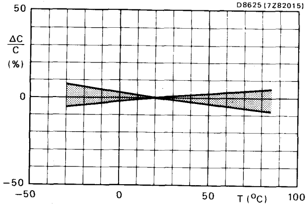
Fig.5 Characteristic V (2B2, Y5F)
