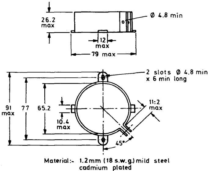
Fig.4 Clamp for case diameter of 65 mm Type No. DT2400
