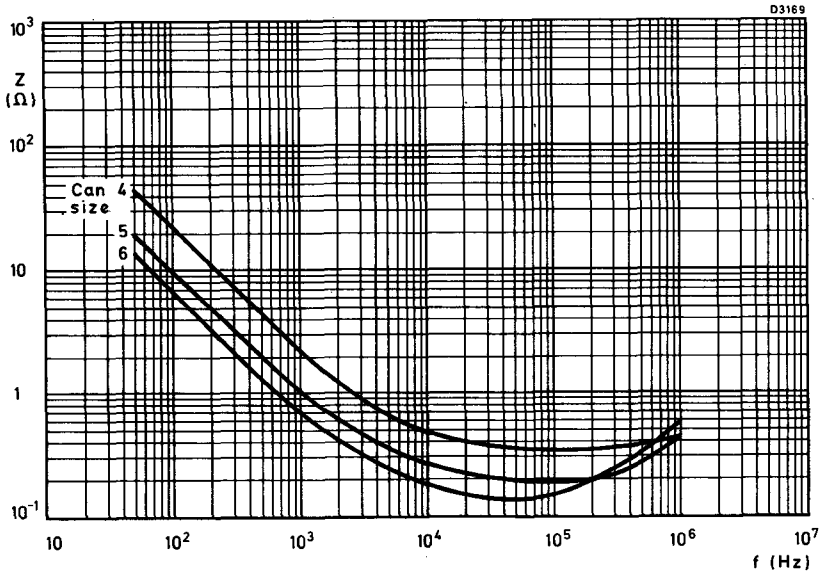
Fig.7 Typical impedance plotted against frequency, T_{amb} = 20^{\circ}C .
