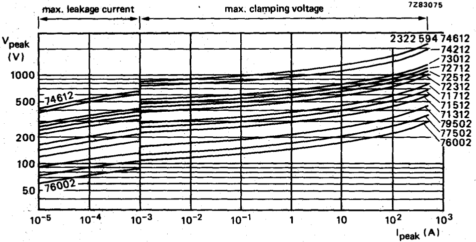
Fig.2 V/I characteristics
