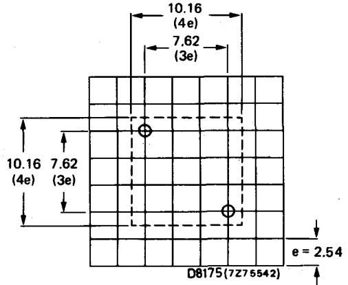
Fig.4 Required space for capacitors according to Fig.2
