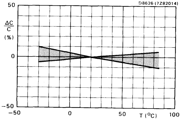
Fig.6 Characteristic SB (2B4, Y5P)
