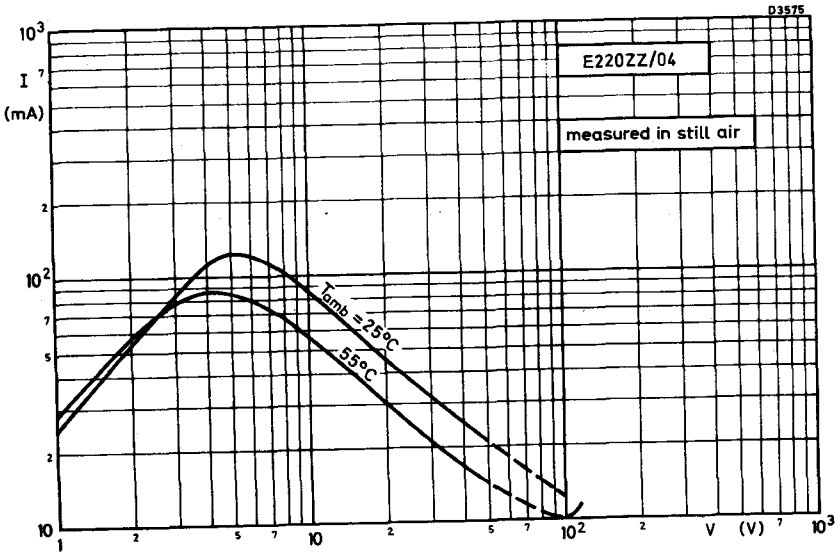
VOLTAGE/CURRENT CHARACTERISTICS
