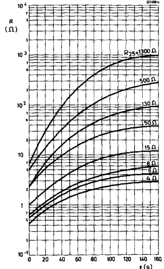
Cooling characteristics
