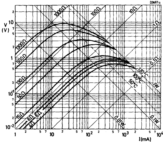
Voltage/current characteristics
