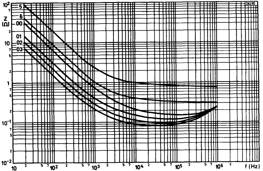
Typical impedance plotted against frequency for 16 V working capacitors, T_{amb} = 20\text{ }^{\circ}\text{C} Can sizes 00, 01, 02, 03, 5 and 6.
