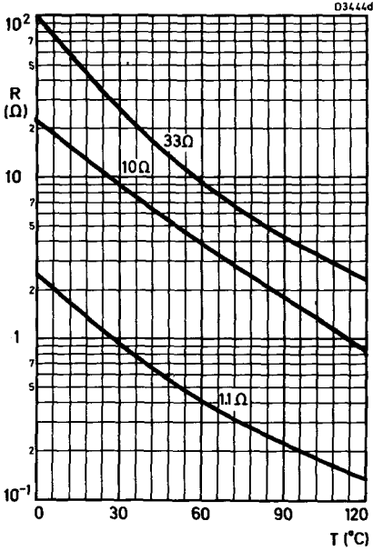
Resistance/temperature characteristics
