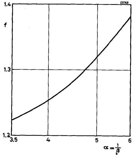
Fig. 8 Factor f by which the mean current value must be multiplied to obtain the r.m.s. current
