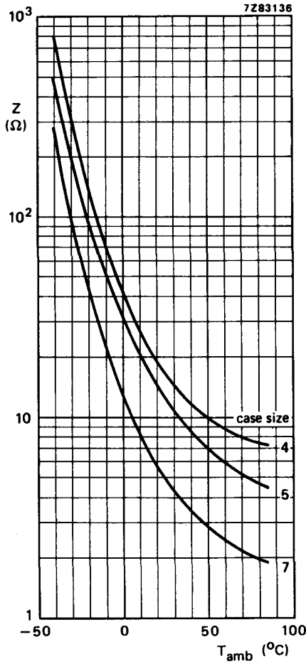
Fig. 9 Typical impedance as a function of ambient temperature at 10 kHz; U_R = 250 V.
